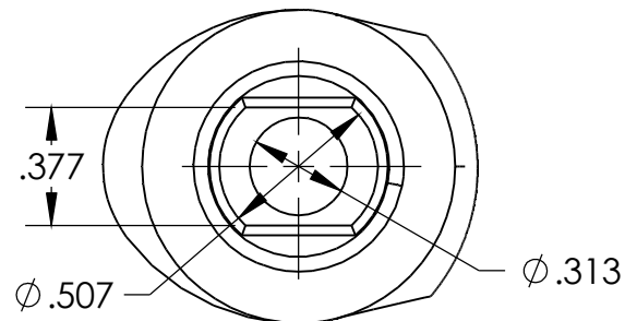
DETAIL A SCALE 3 : 2 (REGULATOR DRIVE)
