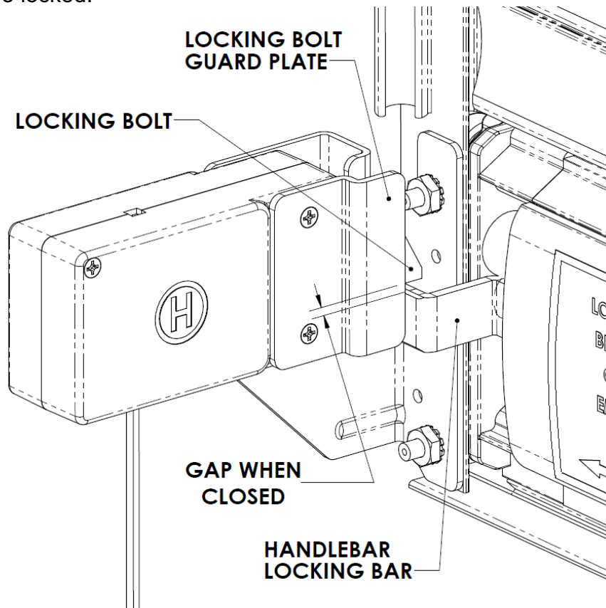
Fig. 27 – E-lock functionality
